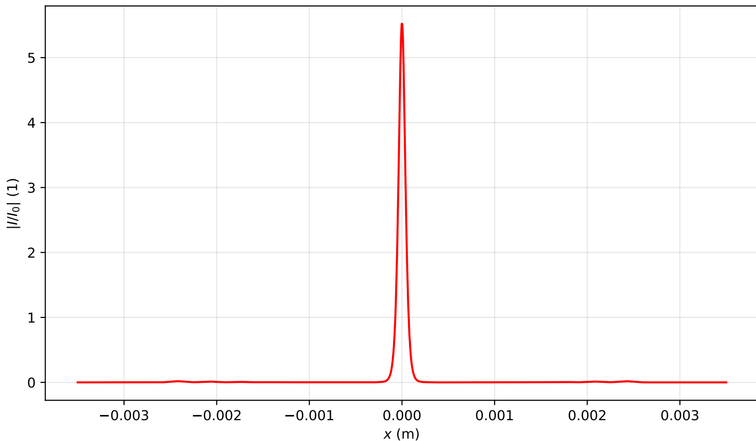
Intensity profile I(x, y = 0, z = 2.229)/I_0 , P_{in}=8.0P_{cr} , artificial time
